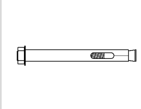
19 M12 x 115mm Galvanised Dynabolts
